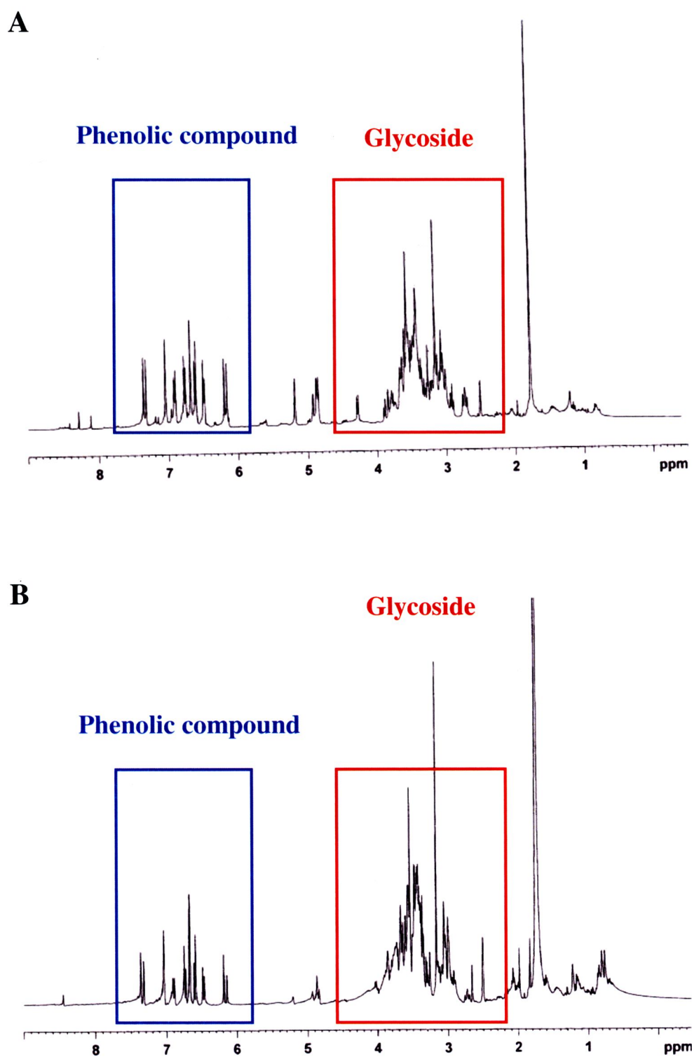
Figure 8 NMR spectra of the 13 th fraction (A) and the 14 th fraction (B) of T. laurifolia leaf extract showing contents of phenolic and glycoside compounds
