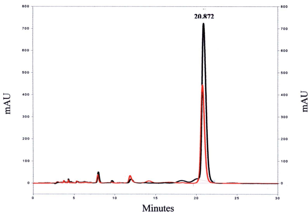
Figure 18. HPLC chromatogram is shown the retention time at 20.872, as same as, standard \alpha -mangostin from Sigma-Aldrich® (USA). The black line was standard \alpha -mangostin and the red line was xanthone, used in this study.
