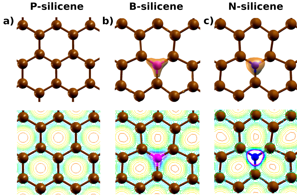
Figure 3.4: Charge density for (a) pristine silicene; (b) B-doped silicene and (c) N-doped silicene. The plotted isosurface corresponds to a value of 0.08e \times bohr^{-3} for all panels.
