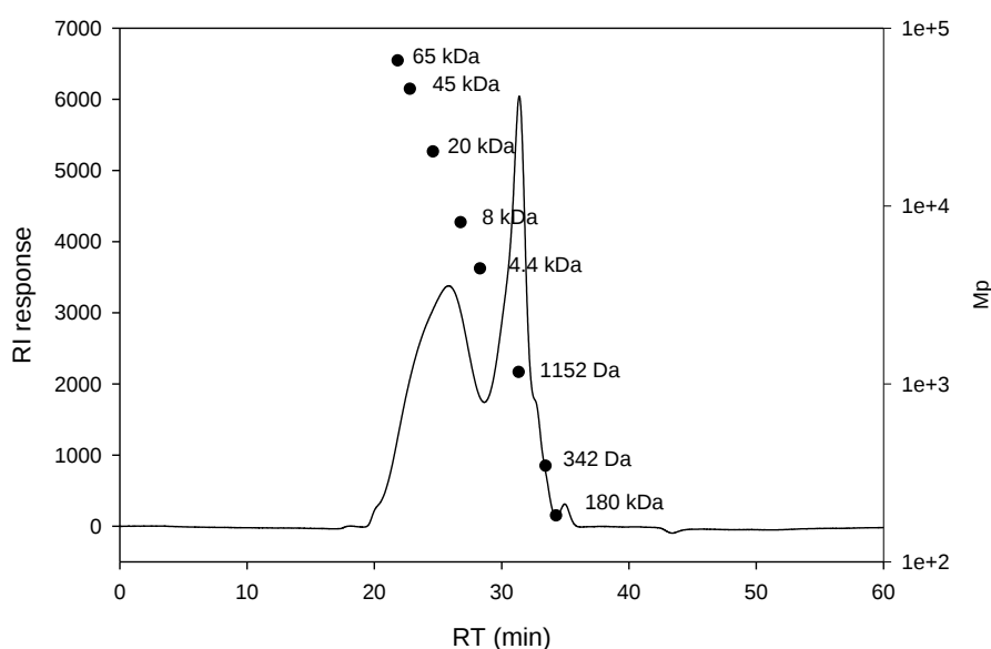
Figure 3 Chromatogram of tapioca maltodextrin with DE6 analyzed with column High Performance Liquid Chromatography (HPSEC).
