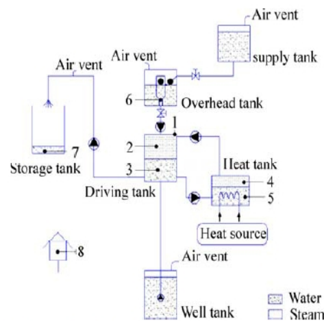
Fig. 3 Locations of temperature and pressure measurement in 10 L pump (1–Pressure of DT; 2–Steam temperature in DT; 3–Water temperature in DT; 4–Steam temperature in HT; 5–Water temperature in HT; 6–Water temperature in OT; 7–Water temperature in ST; 8–Ambient temperature)
