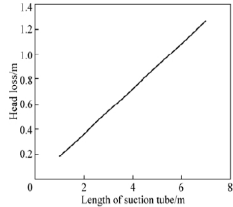
Fig. 13 Effect of length of suction tube on head loss
