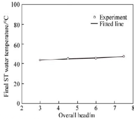
Fig. 11 Final ST water temperature from experiment as a function of overall head for 10 L pump
