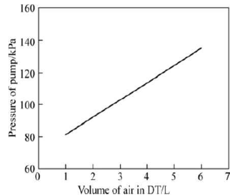
Fig. 10 Effect of air volume within DT on pumping pressure
