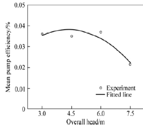
Fig. 14 Mean pump efficiency from experiment and fitted line based on Eq. (14) as a function of overall head for 10 L pump (Root-mean-square error is 0.0582%)
