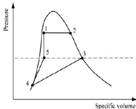
Fig. 7 P–V diagram of a pumping process
