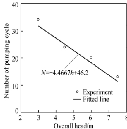
Fig. 15 Number of pumping cycle N from experiment as a function of overall head in 2 h for 10 L pump (Root-mean-square error is 6.42%)
