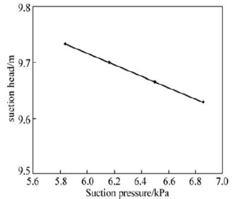
Fig. 19 Effect of suction pressure on suction head
