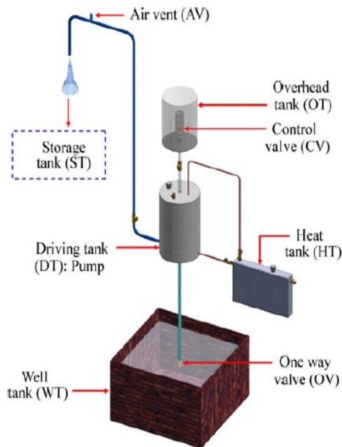
Fig. 1 Water pumping system with 10 L capacity
