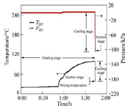
Fig. 17 Mean temperature in DT ( T_{DT} ) and gage pressure in DT ( P_{DT} ) as a function of time for suction head 3 m (200 L pump with one-cycle operation, experimental study)
