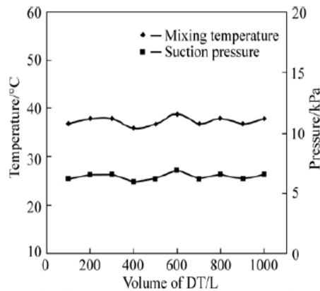
Fig. 18 Effect of DT volume on suction pressure and mixing temperature of cooling stage according to Eqs. (5)–(6)
