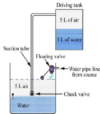
Fig. 5 Air addition to DT
