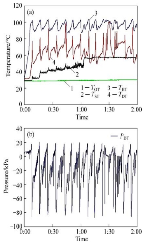
Fig. 9 Water temperature in OT ( T_{OT} ), mean temperature in ST ( T_{ST} ), mean temperature in HT ( T_{HT} ), mean temperature in DT ( T_{DT} ), gage pressure in DT ( P_{DT} ) as a function of time for suction head 6.5 m (10 L pump, present system): (a) Temperature; (b) Pressure
