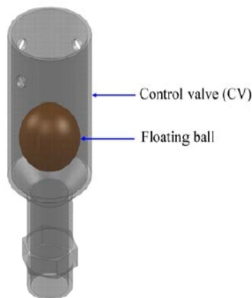
Fig. 2 Schematic diagram of CV
