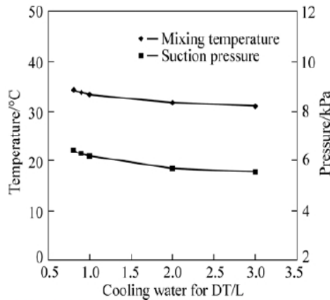
Fig. 12 Effect of a cooling water on mixing temperature and DT suction pressure
