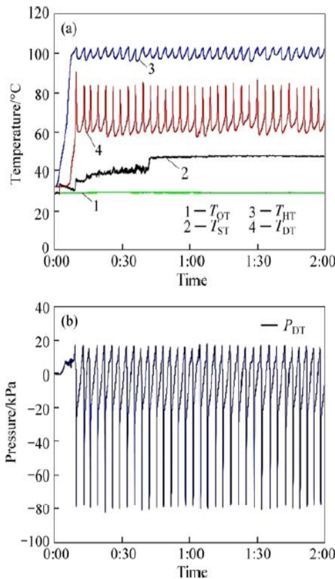
Fig. 8 Water temperature in OT ( T_{OT} ), mean temperature in ST ( T_{ST} ), mean temperature in HT ( T_{HT} ), mean temperature in DT ( T_{DT} ), gage pressure in DT ( P_{DT} ) as a function of time for suction head 2.0 m (10 L pump, present system): (a) Temperature; (b) Pressure
