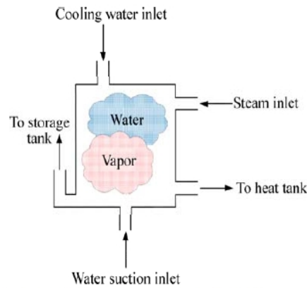
Fig. 6 Schematic diagram of fluid flow within DT
