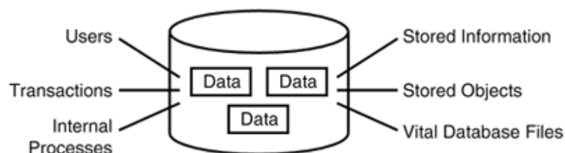
Figure 2.1 The database.
