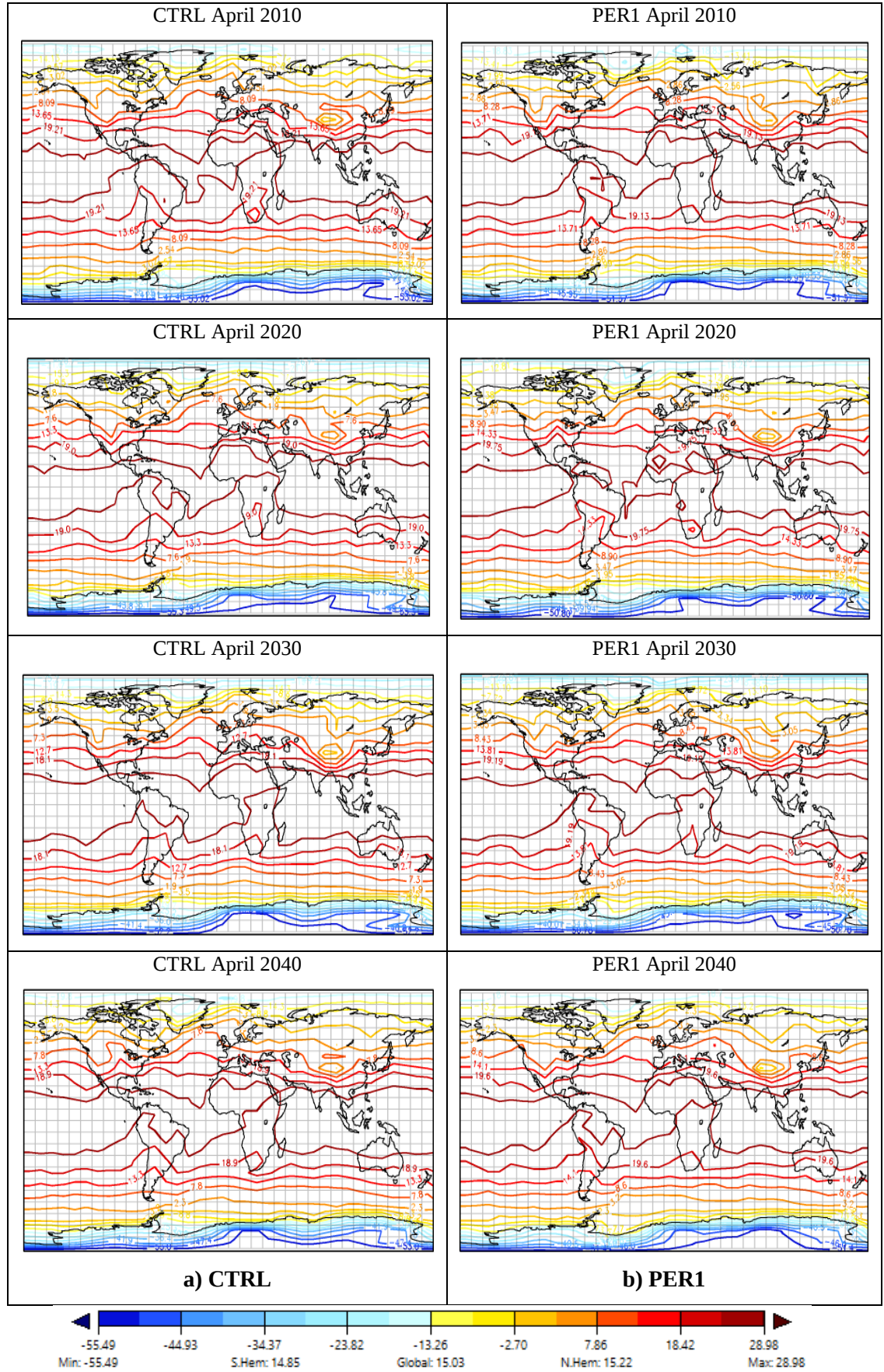
Figure A.1 Forecast surface air temperature in April from EdGCM model for a) CTRL and b) PER1.
