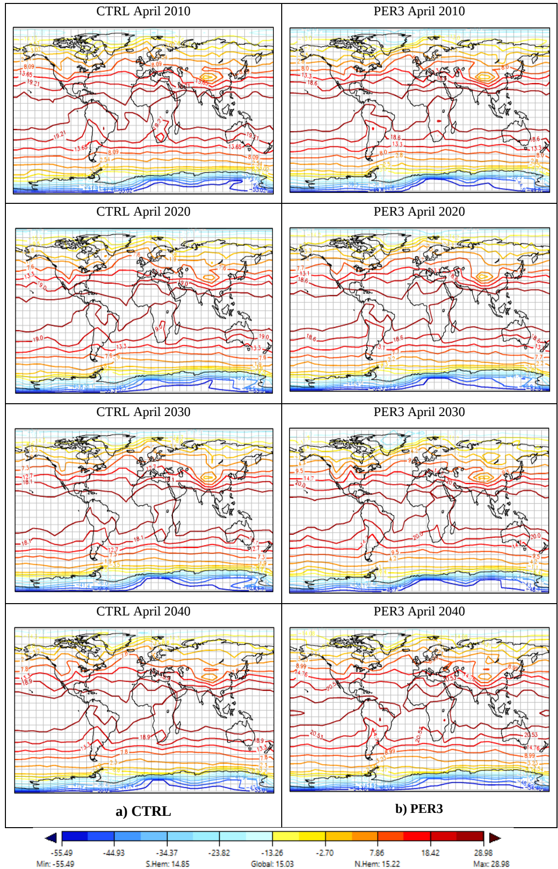
Figure A.3 Forecast surface air temperature in April from EdGCM model for a) CTRL and b) PER3.
