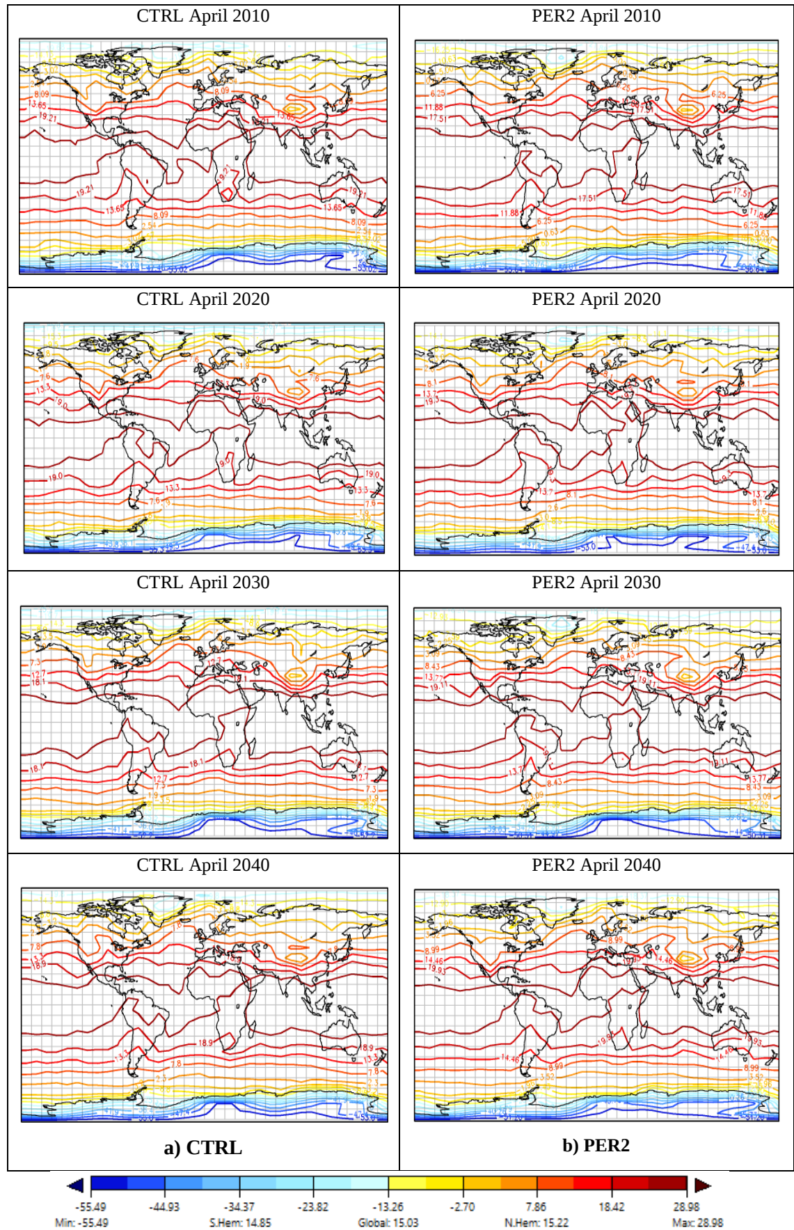
Figure A.2 Forecast surface air temperature in April from EdGCM model for a) CTRL and b) PER2.
