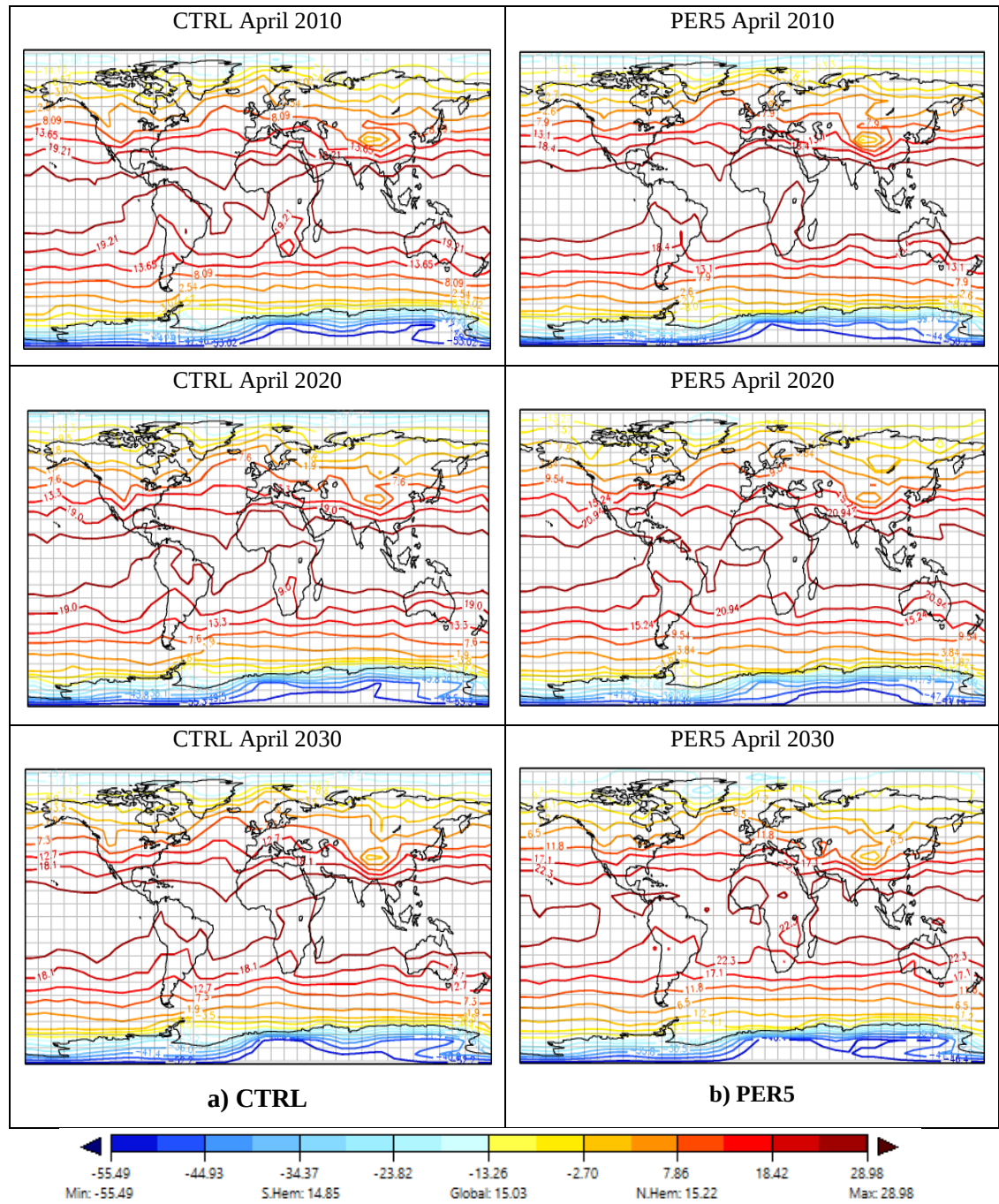
Figure A.5 Forecast surface air temperature in April from EdGCM model for a) CTRL and b) PER5.
