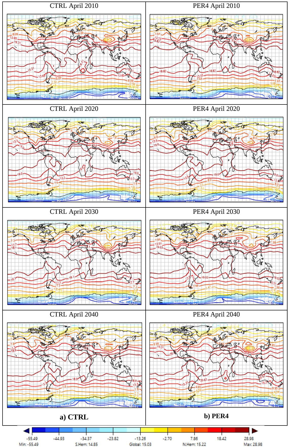
Figure A.4 Forecast surface air temperature in April from EdGCM model for a) CTRL and b) PER4.
