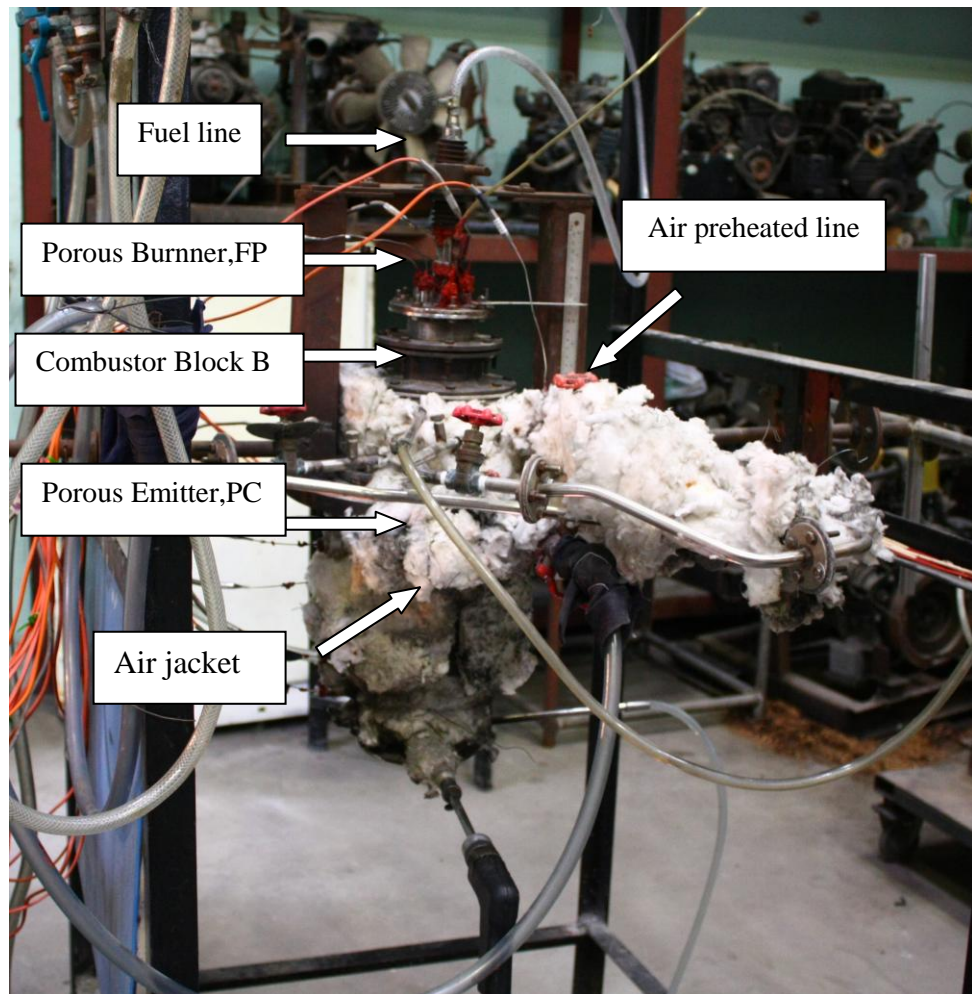
Figure A.1 Modulating dual fuel porous burner (MDPB).
