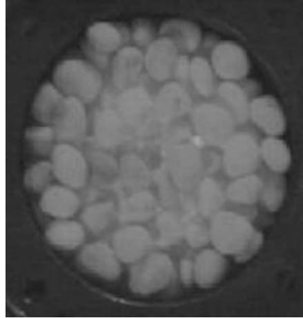
Figure A.3 Packed bed of Al 2 O 3 (PC).
