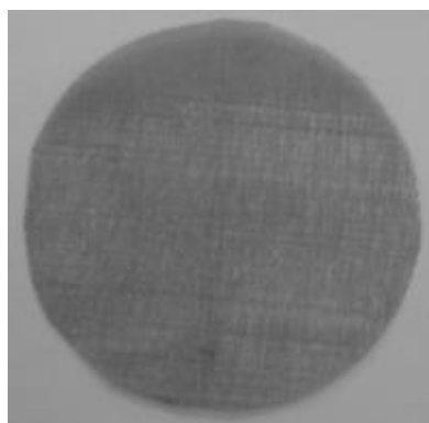
Figure A.2 100 mesh/inch stainless wire screen (FP).
