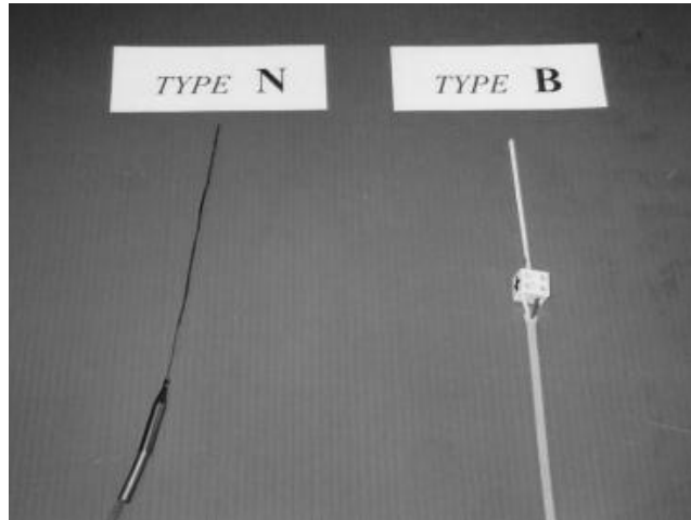
Figure A.6 N-type and B-type thermocouples.
