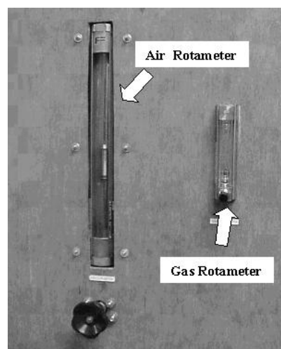
Figure A.5 Rotameter.
