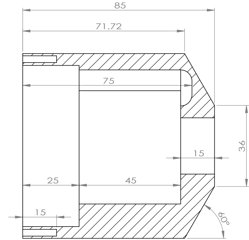
SECTION C-C
