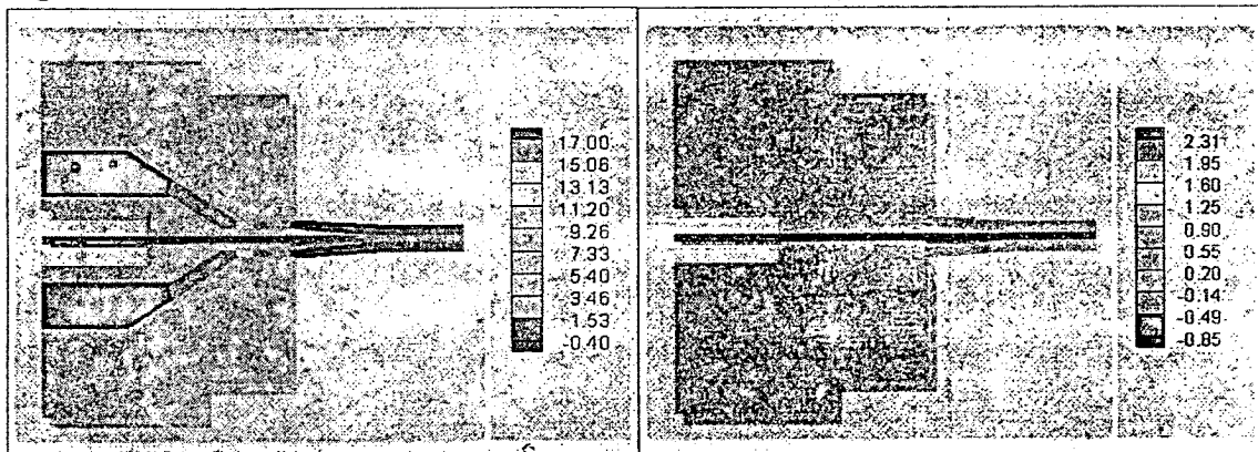
Figure 7. Color contour of We=200 for (a) radial velocity u_r , (b) axial velocity v_z
