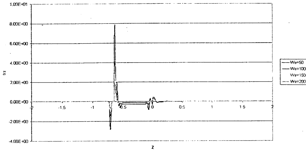
(c) Shear stress T_{rz} at top surface
