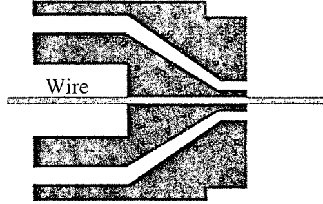
Figure 3: Schema of tube-tooling die
