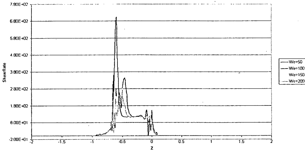
(a) Shear rate at top surface
