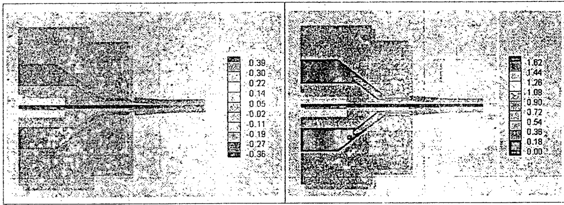
(b) Axial velocity v_z
