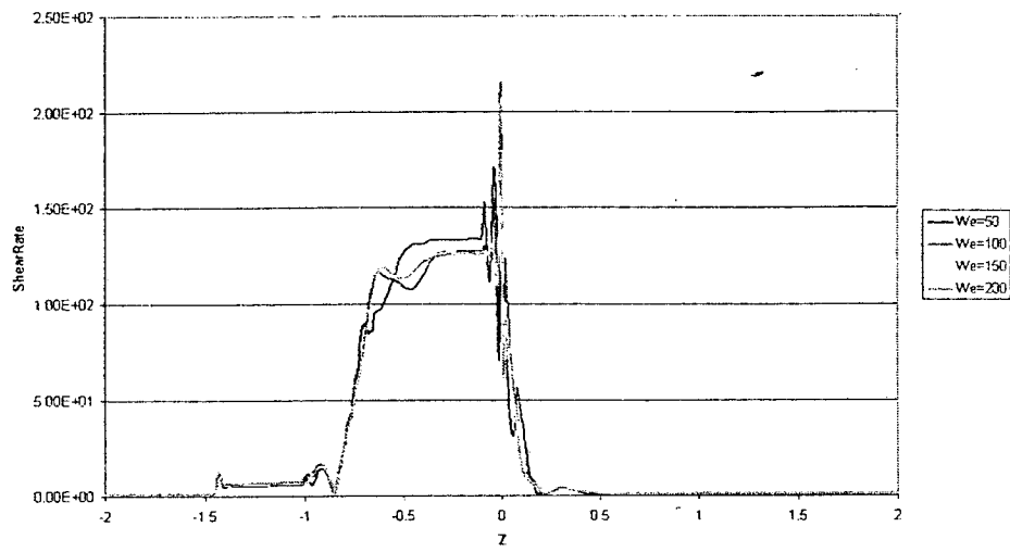
(a) Shear rate at bottom surface
