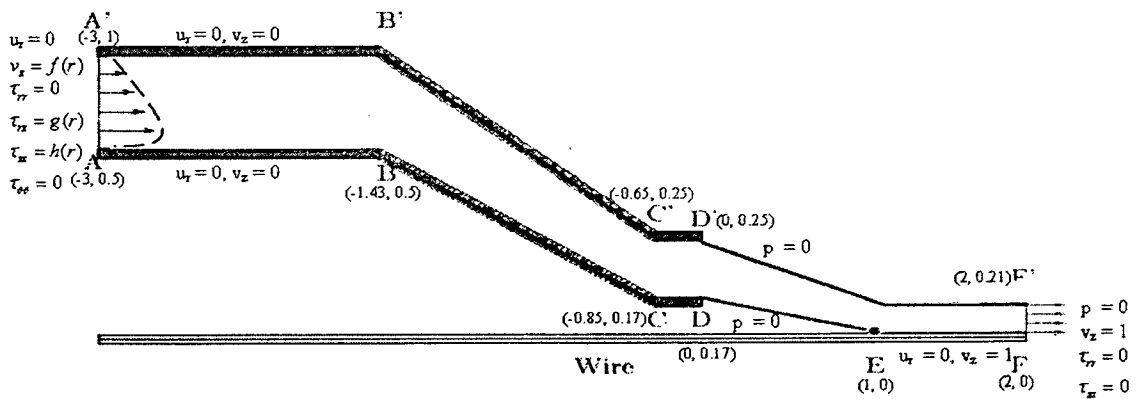
Figure 5: Schema of boundary domain
