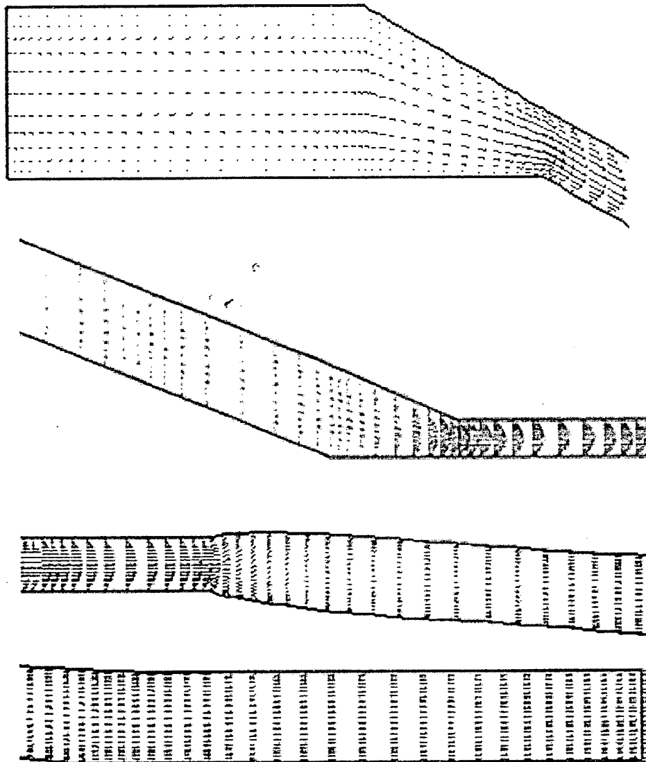
Figure 6. Velocity vector
