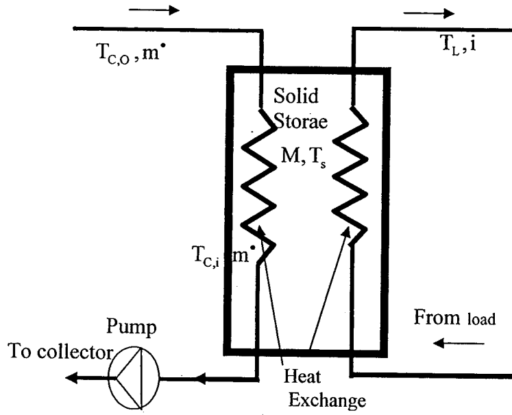
Figure 16 Fully mixed storage with heat exchangers
