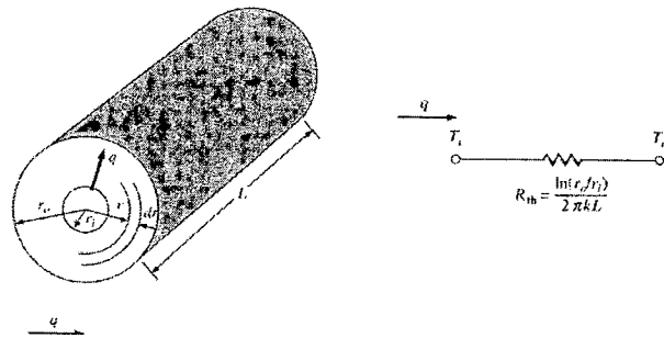
Figure 13 One-dimensional heat flow through a hollow cylinder and electrical analog
