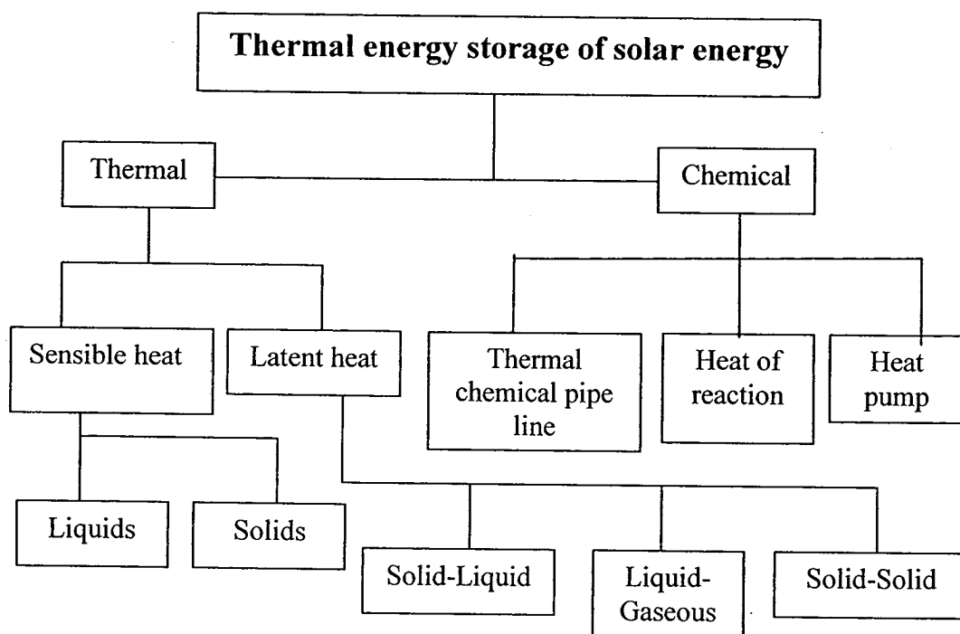
Figure 8 Storage of solar thermal energy
