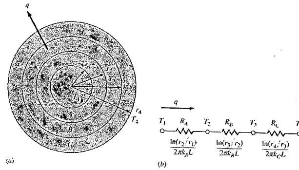
Figure 14 One-dimensional heat flow through multiple cylindrical section and electrical analog
