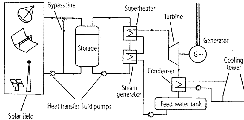
Figure 1 Principle of a solar thermal power plant
