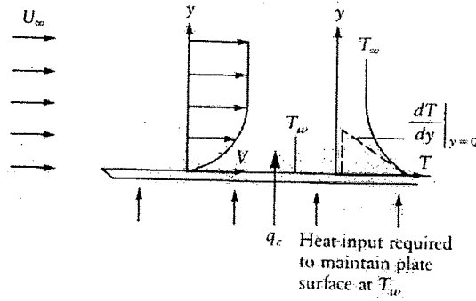
Figure 11 Uniform flow past a heated plate
