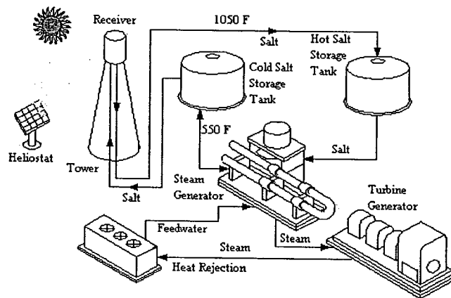
Figure 2 Molten salt power tower system schematic diagram
