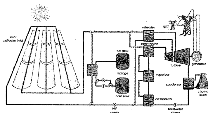
Figure 9 Schematic of a concentrated solar thermal trough power plant with thermal storage
