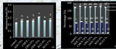
Figure 7 Texture (a) and cooking quality (b) of Ubon noodles with hydrocolloids.
