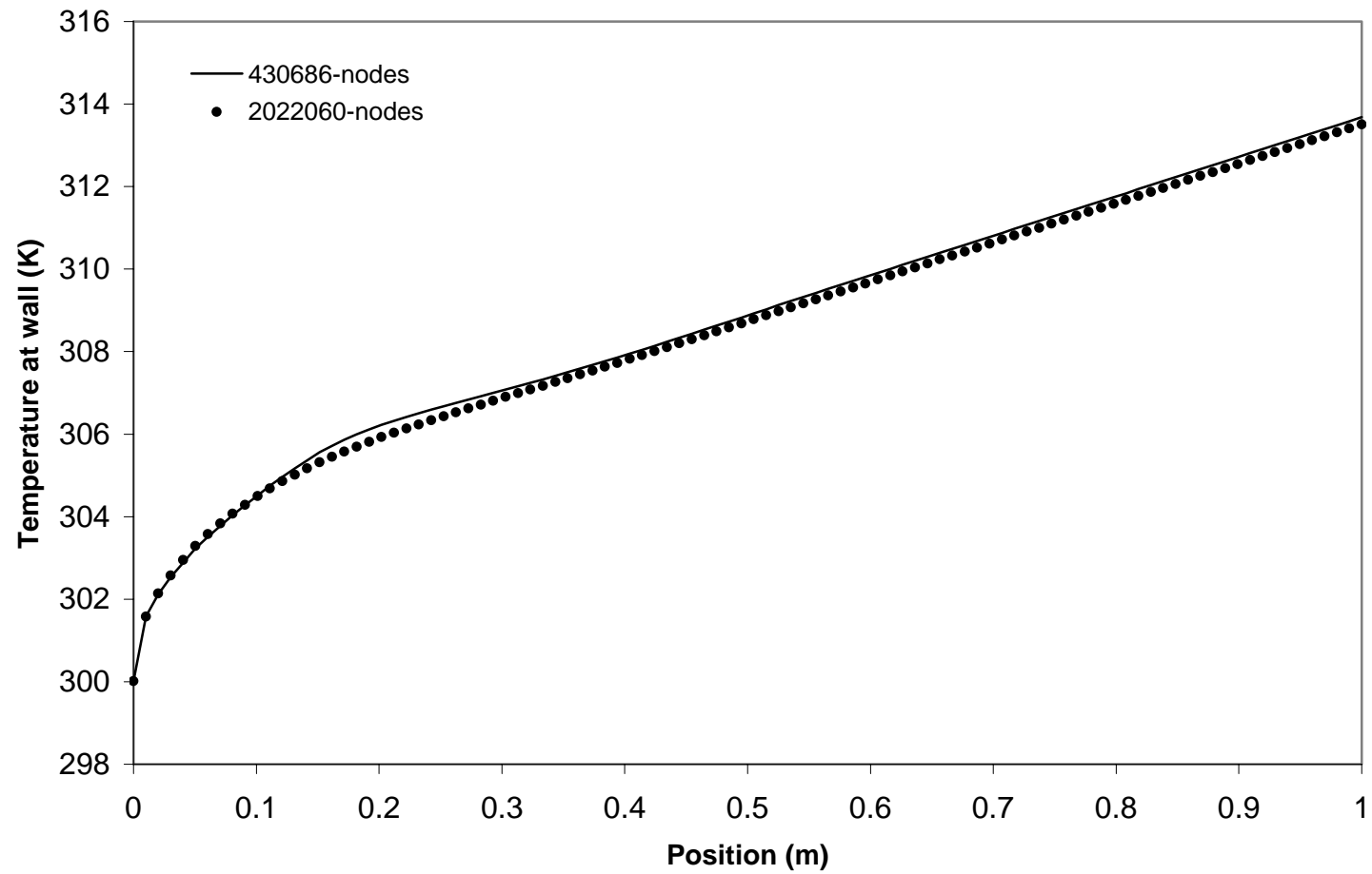
Figure 4 Results of grid sensitivity study
