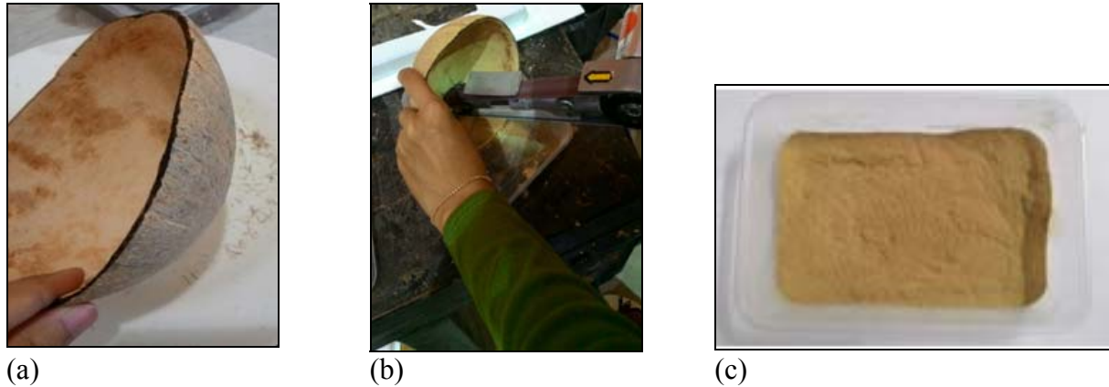
Figure 1. Preparation of the based material (a) Cleaned and well dried coconut shell, (b) Sanding process and (c) Coconut shell powder
