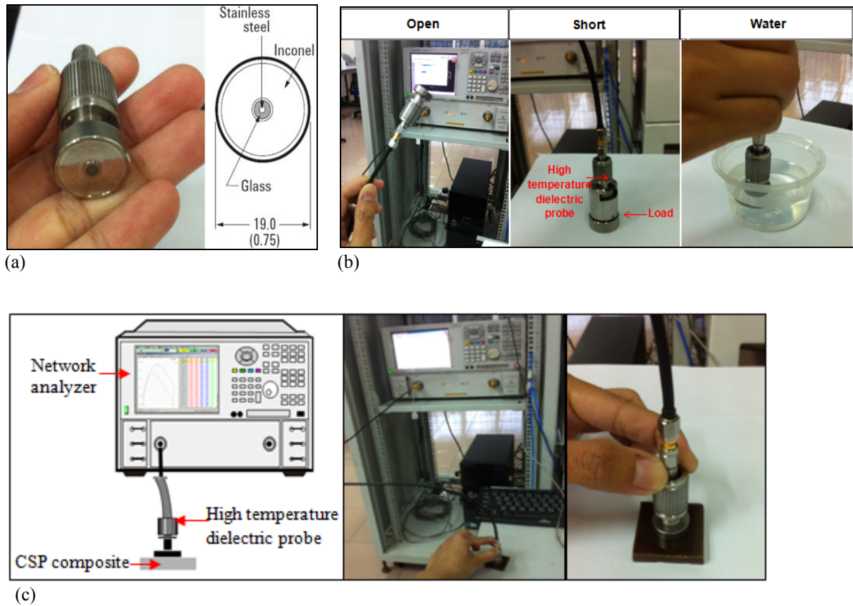
Figure 3. Measurement apparatus (a) High temperature dielectric probe, (b) Three standard calibration and (c) Dielectric properties measurement setup by using open-ended coaxial probe method
