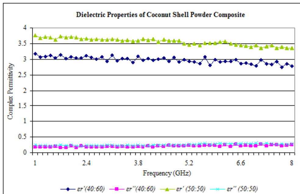
Figure 6. Dielectric properties of coconut shell powder composites
