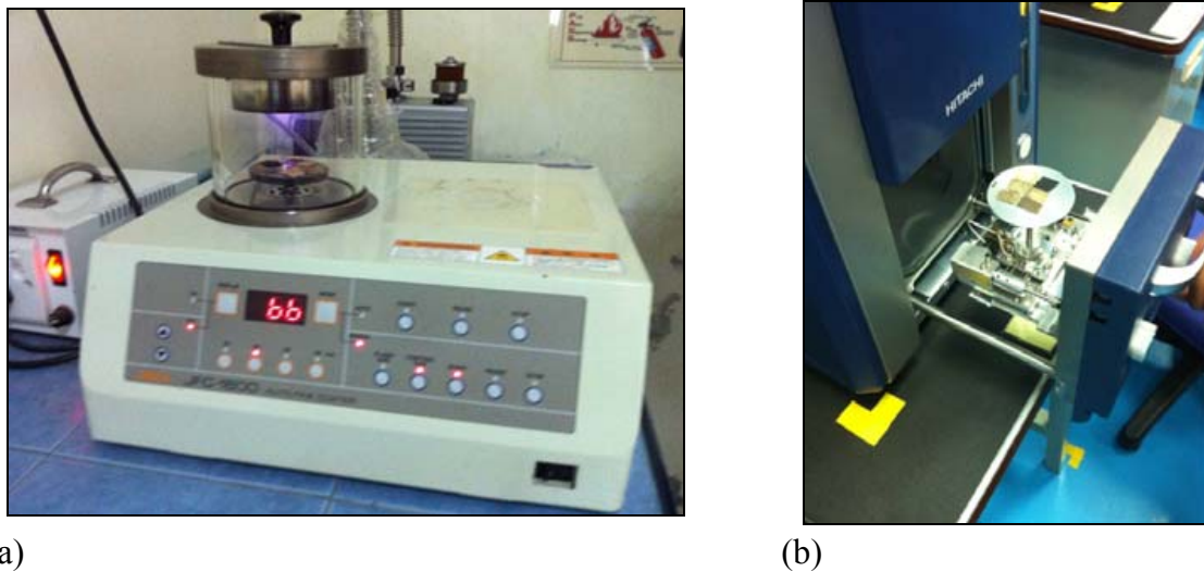
Figure 2. (a) Coating of coconut shell powder sample with platinum (JFC 1600 Auto Fine Coater), (b) Placement of the sample on the specimen holder (Hitachi TM3000 Tabletop microscope)
