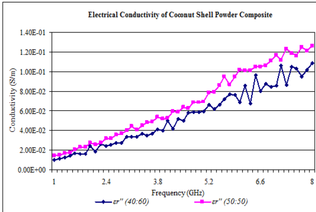
Figure 7. Conductivity of coconut shell powder composites
