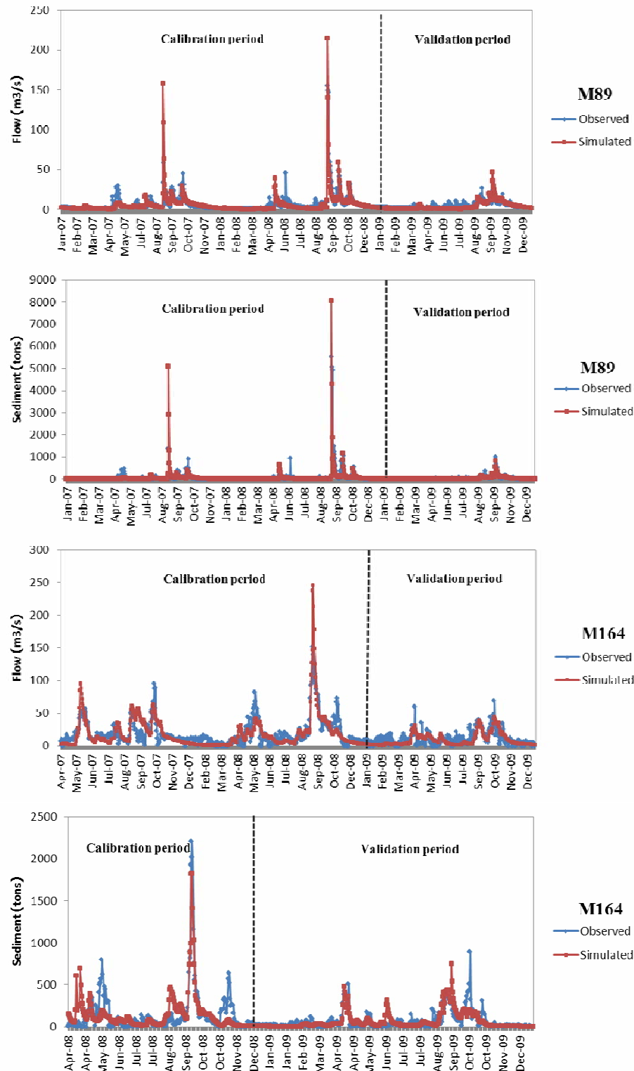
Figure 3. Comparison between the simulated and observed streamflow and sediment values of M89 and M164
