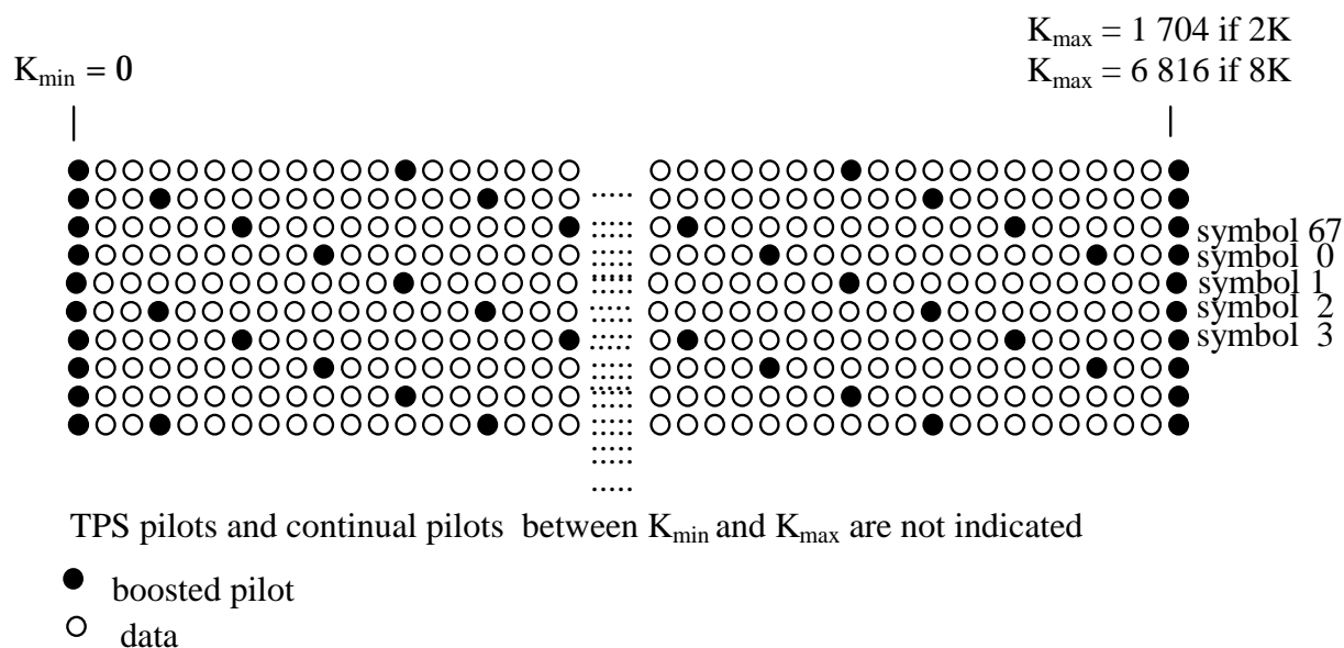
Figure 11: Frame structure
