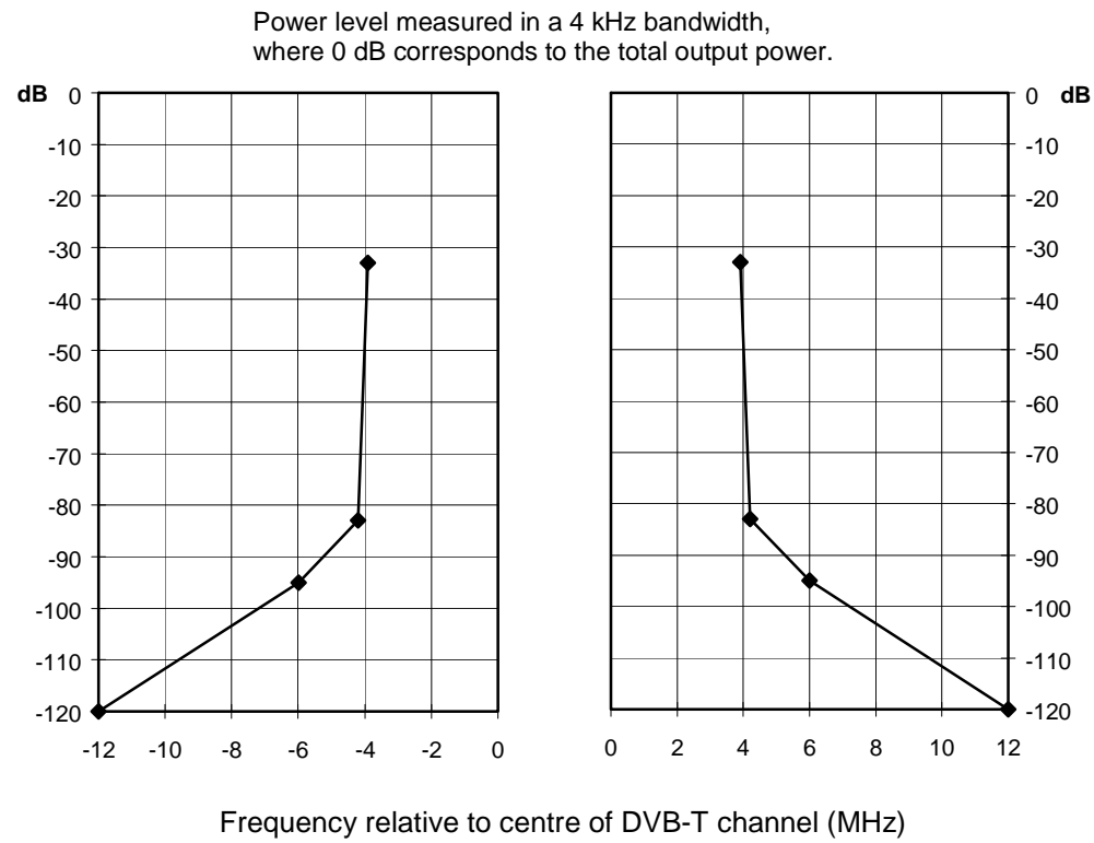
Figure 14: Spectrum mask for critical cases
