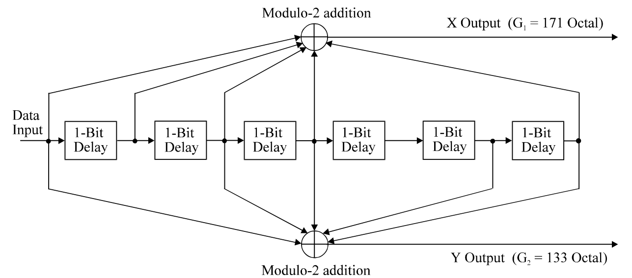
Figure 5: The mother convolutional code of rate 1/2
