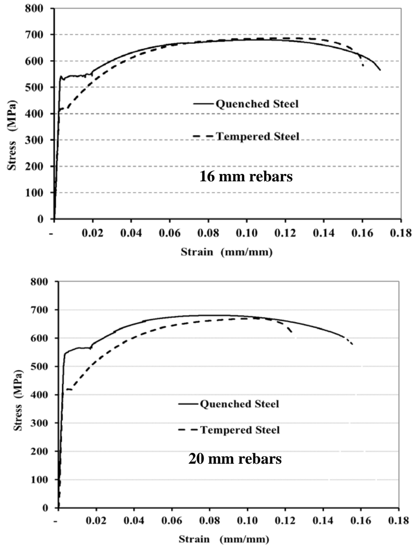
Figure 1. Typical stress-strain curves for 16 mm and 20 mm rebar.
