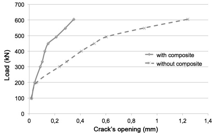
Figure 3. Positive local effect preventing cracks from widening thanks to composite.
