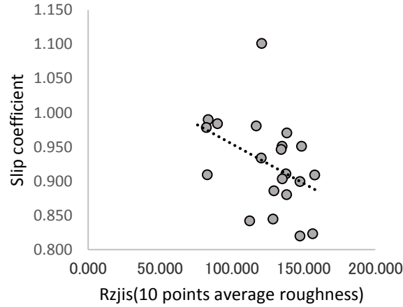
Figure 6. Relationship between slip coefficient and Rzjis.
