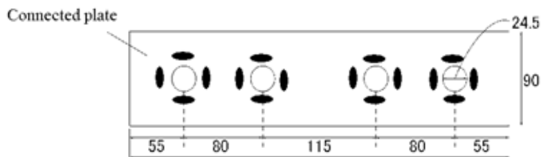
Figure 2. Example of measurement position (splice plate) [unit: mm].
