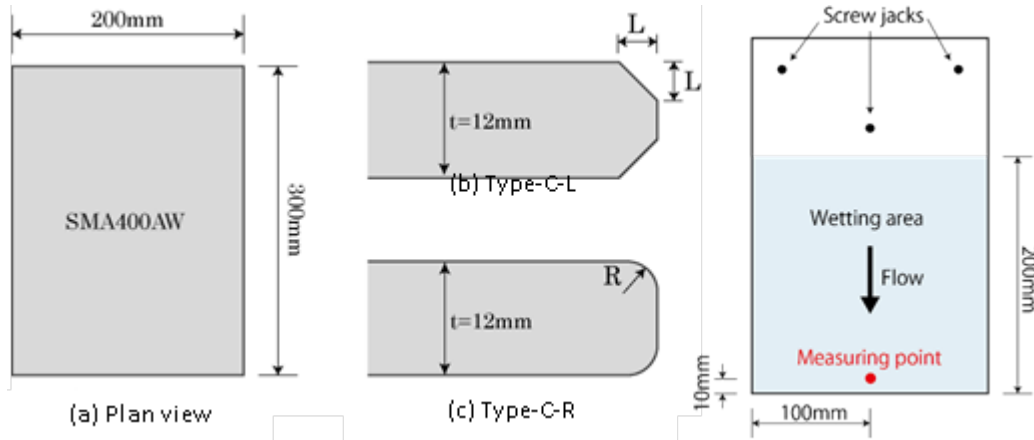
Figure 1. Dimensions of specimen.
