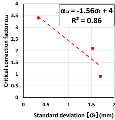
Figure 6. \alpha_{cr} - \sigma_t relationship.
