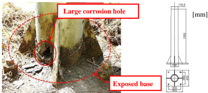
Photo 1. In-situ condition and dimensions of road-lighting pole specimen.
