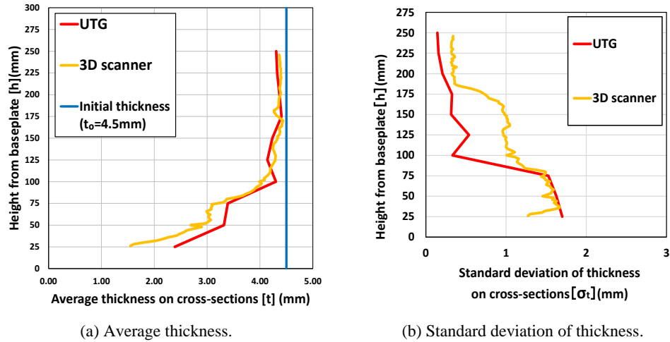
Figure 3. Relationship between h and statistical thickness parameters.
