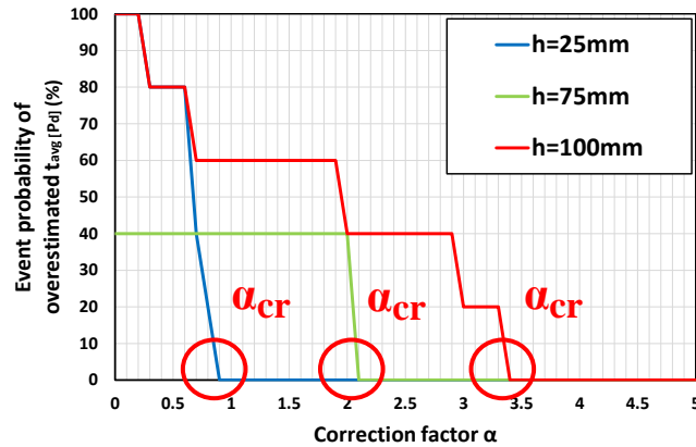
Figure 4. Event probability of overestimated P_d .
