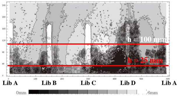
Figure 1. Thickness contour map (3D scanner).
