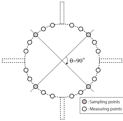
Figure 5. A measuring unit with 4 sampling points.
