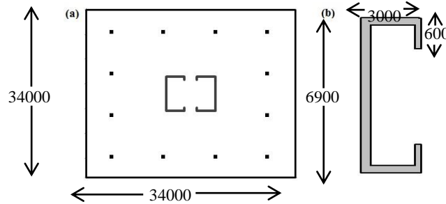
Figure 1. (a) Plan view of building with central core. (b) Dimensions of the C-shaped walls.
