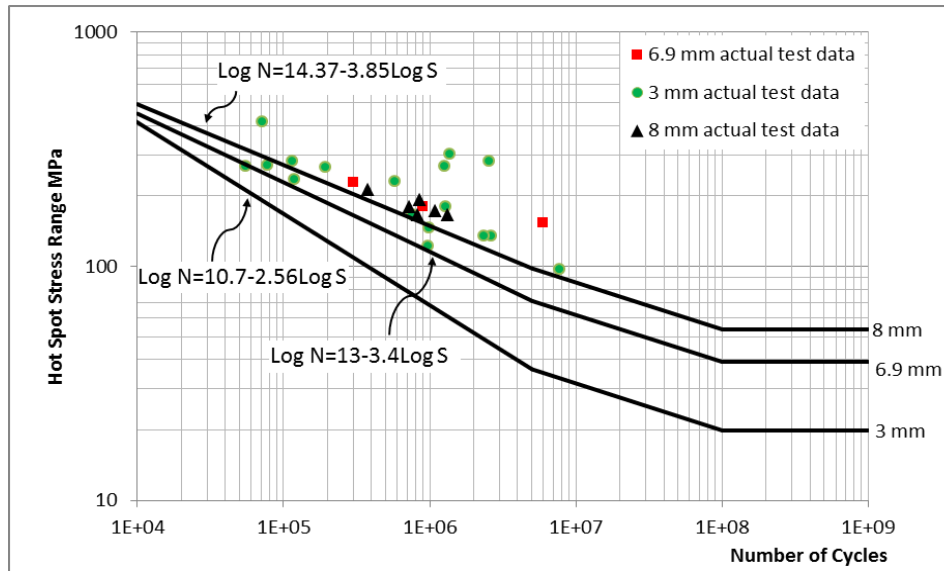
Figure 4. Hot spot stress design curves.
