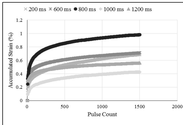
Figure 2. Relationship between accumulated strain (%) and pulse count.
