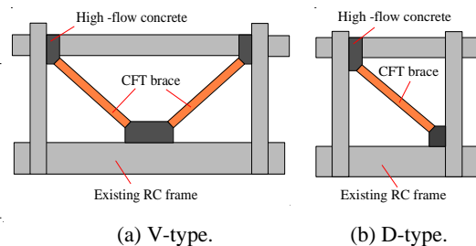
Figure 2. Elevations of the retrofitted frames.
