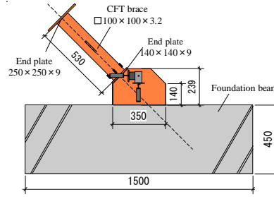
Figure 7. Elevation (35-45DB).
