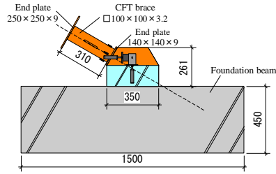
Figure 6. Elevation (35-30DB).
