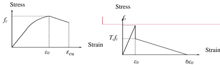
Figure 1. Stress-strain relationship of concrete: (a) compression (Nitereka and Neal 1991); (b) Tension (ANSYS13.0).
