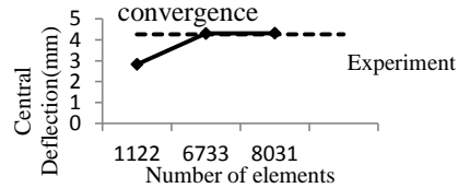
Figure 3. Convergence test for the control beam.
