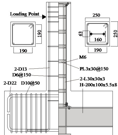
Figure 2. Test specimen
