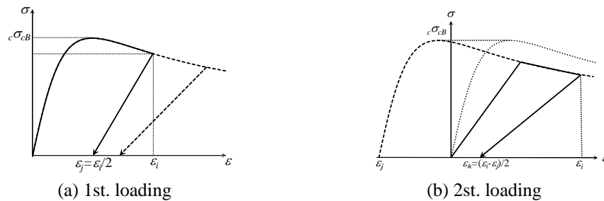
Figure 5. Stress-strain relation of concrete.
