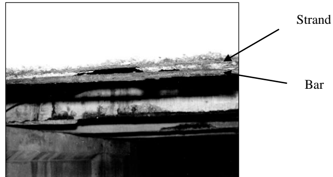
Figure 4. Prestressed concrete roof elements ECP: cracking and spalling of the concrete cover; advanced corrosion of the non-pre-tensioned bar and pre-tensioned strand.
