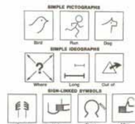
Sigsymbols
